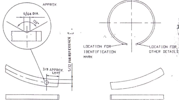
ENLARGED DETAIL OF OPTIONAL PIT MARK FOR M/S KAYDON RINGS.
