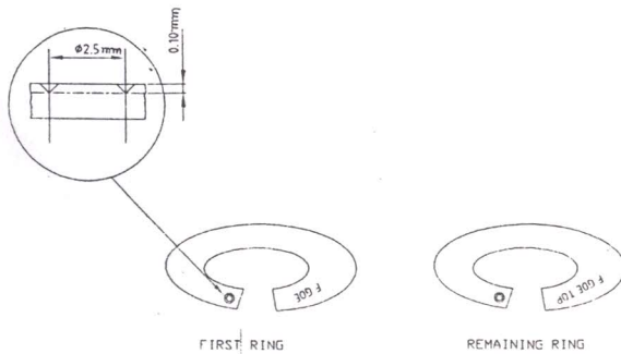
DETAIL OF IDENTIFICATION MARK OF M/S GOETZE.
